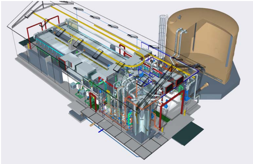
detail design membrane bioreactor
